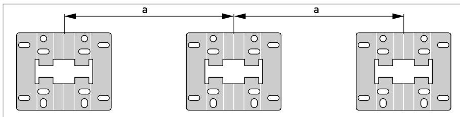
Figure 3-19: Mounting multiple devices next to each other
