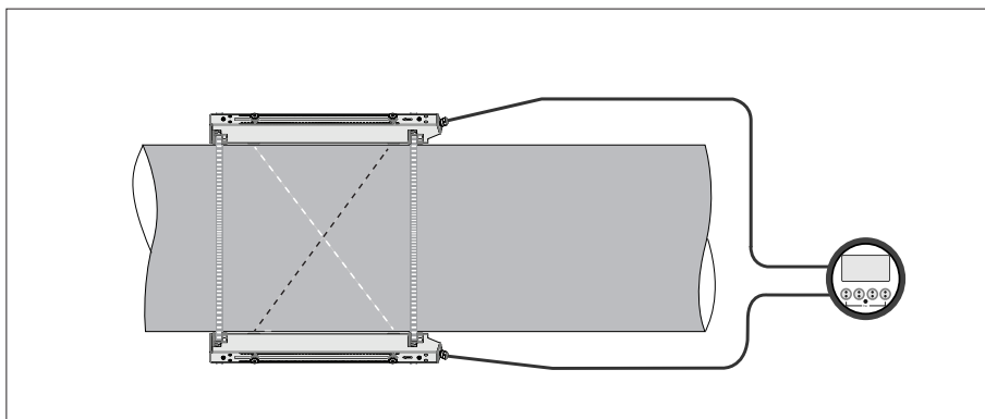
Figure 1-6: X beam configuration of medium version
