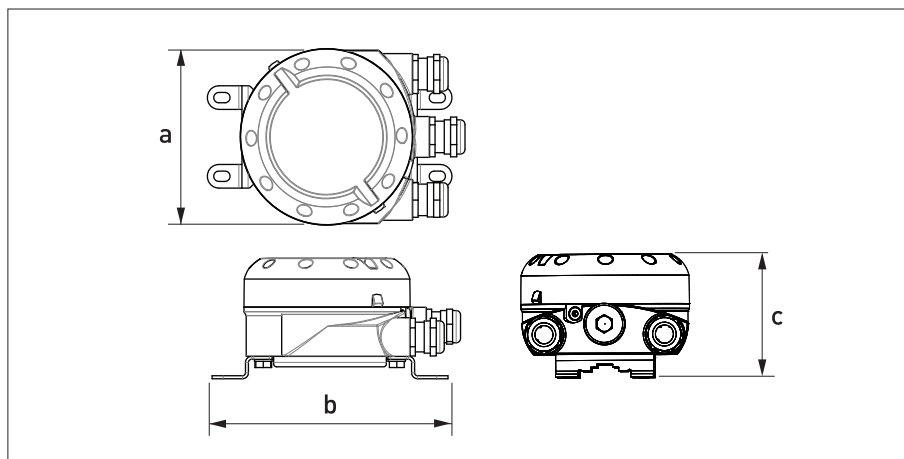
Figure 2-4: Dimensions stainless steel version
