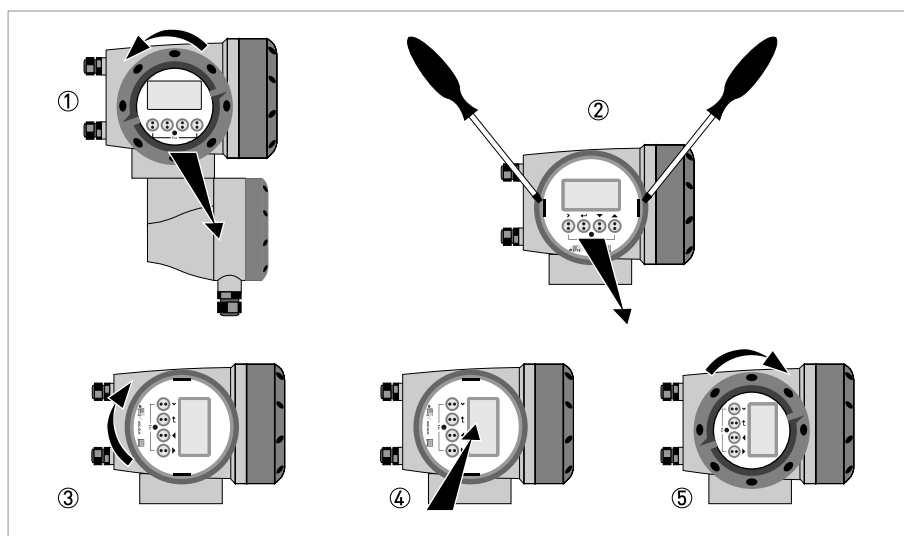
Figure 3-20: Turning the display of the field housing version
