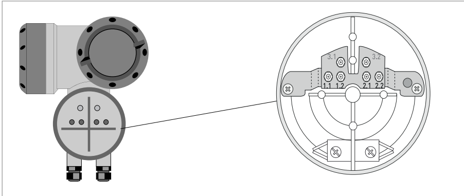
Figure 4-7: Connect signal cable
