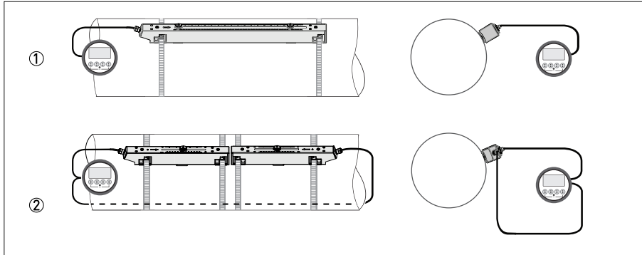
Figure 1-2: Overview of single path variants
