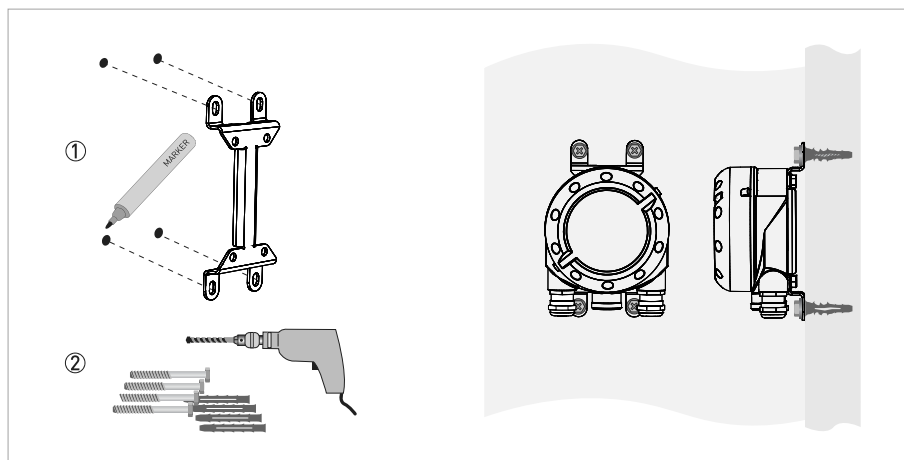
Figure 3-13: Wall mounting
