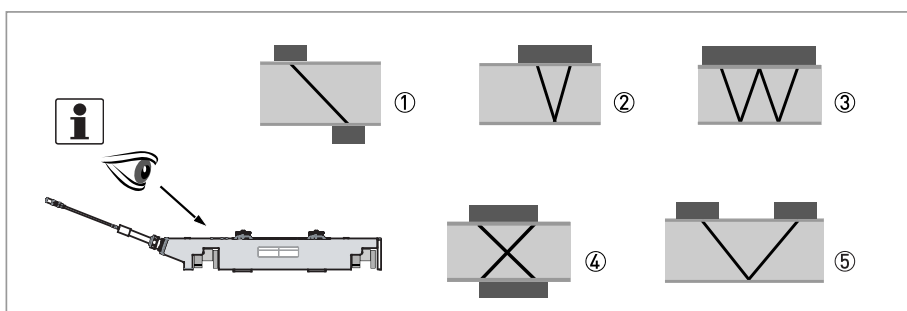
Figure 3-10: Measuring modes
