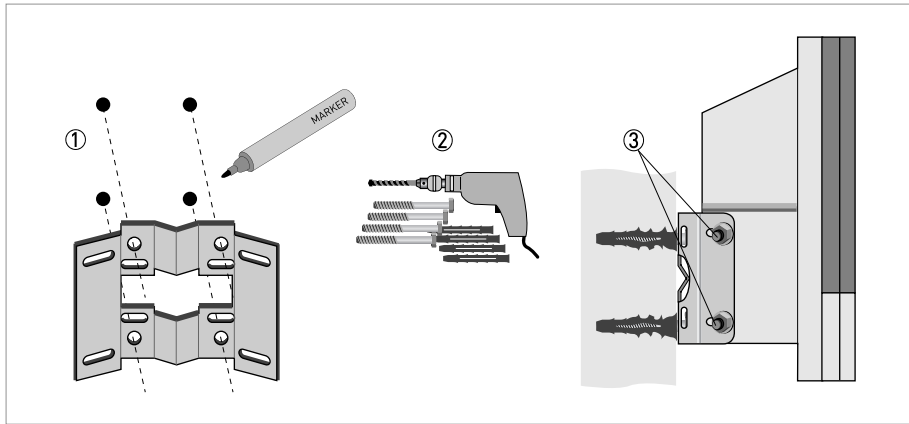
Figure 3-18: Wall mounting of the wall-mounted housing
