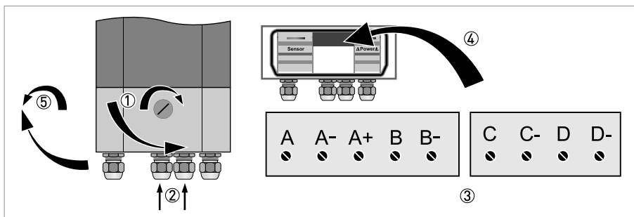
Figure 4-14: Terminal compartment for inputs and outputs of the wall-mounted housing
