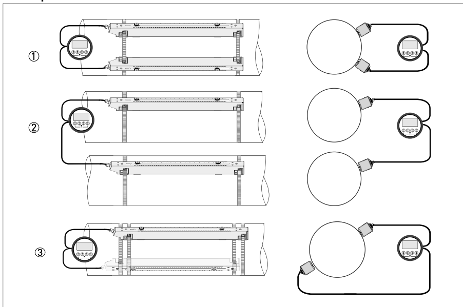
Figure 1-3: Overview of dual-path variants
