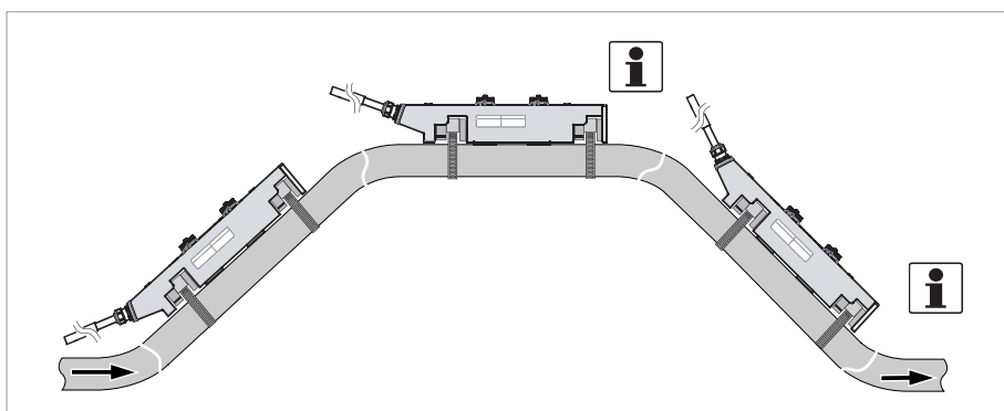
Figure 3-5: Installation in bending pipes (45°)
