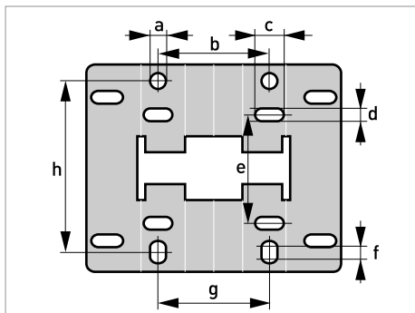
Figure 2-6: Dimensions of mounting plate of wall-mounted housing
