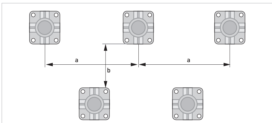
Figure 3-17: Mounting multiple devices next to each other
