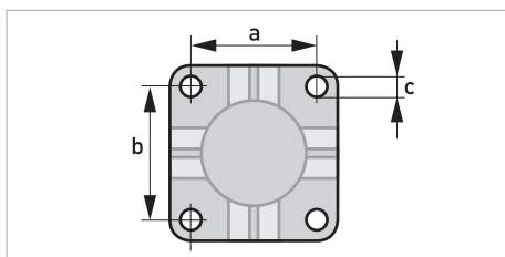
Figure 2-5: Dimensions for mounting plate of field housing
