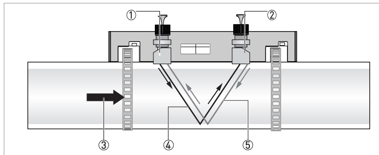
Figure 1-8: Measuring principle (example reflected path set-up)
