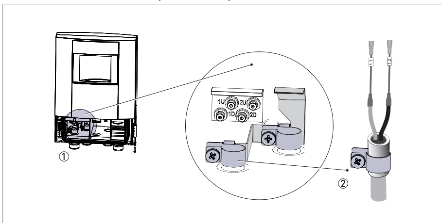
Figure 4-10: Inserting cable and secure with clamp on shielding bush
