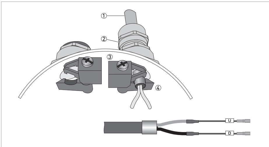
Figure 4-8: Inserting cable and secure with clamp on shielding bush
