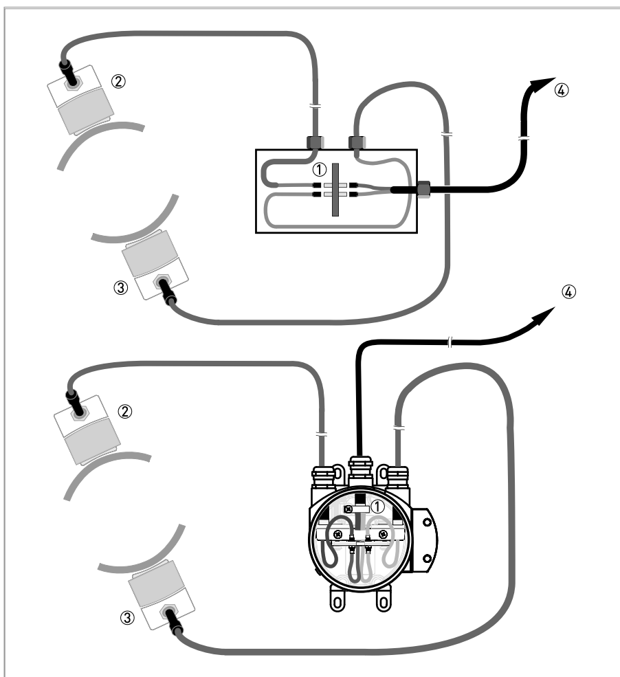
Figure 4-12: Example of large sensor rail connections with cable (splitter) box
