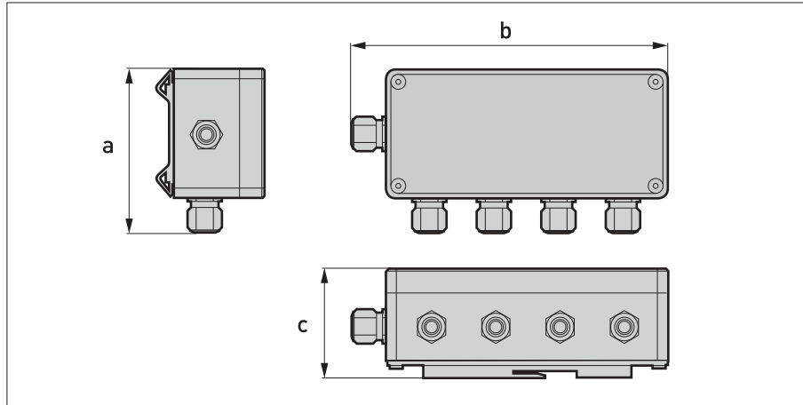
Figure 2-3: Dimensions aluminium version
