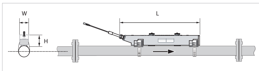
Figure 2-2: Dimensions clamp-on sensor rail(s)
