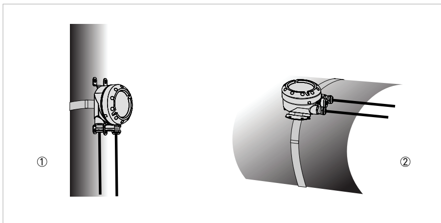
Figure 3-14: Pipe (pole) mounting or installation on the pipe line
