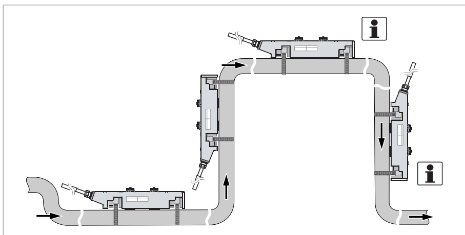
Figure 3-4: Installation in bending pipes (90°)
