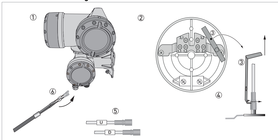
Figure 4-9: Construction of field version
