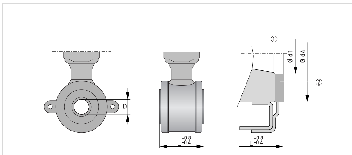
Figure 2-1: Construction details DN25...100
