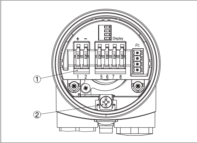
Fig. 17: Electronics and connection compartment, single chamber housing 1 Spring-loaded terminals for power supply 2 Ground terminal for connection of the cable screen
