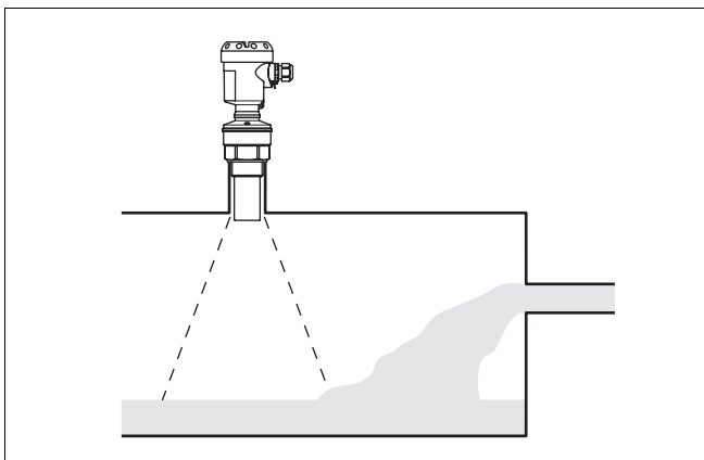
Fig. 13: Inflowing liquid
