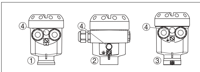
Fig. 16: Material versions, single chamber housing
