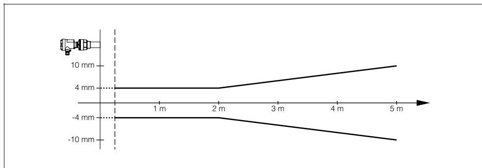
Fig. 25: Accuracy OPTISOUND 3010 C
