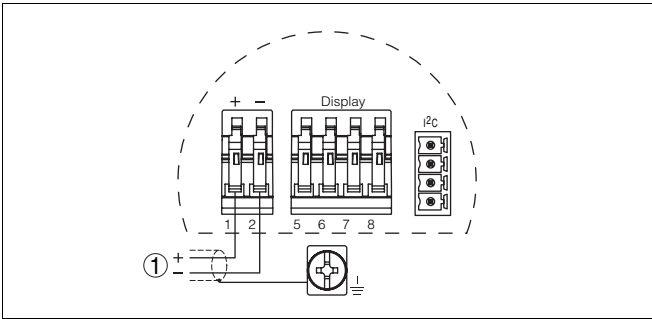
Fig. 18: Wiring plan, single chamber housing 1 Power supply/Signal output
