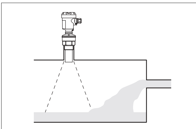
Fig. 13: Inflowing liquid
