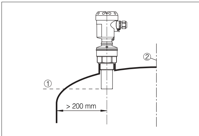
Fig. 5: Mounting on dished vessel tops
