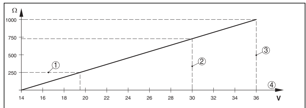
Fig. 23: Voltage diagram
