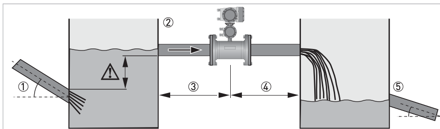
Figure 3-6: Installing in difficult situations
