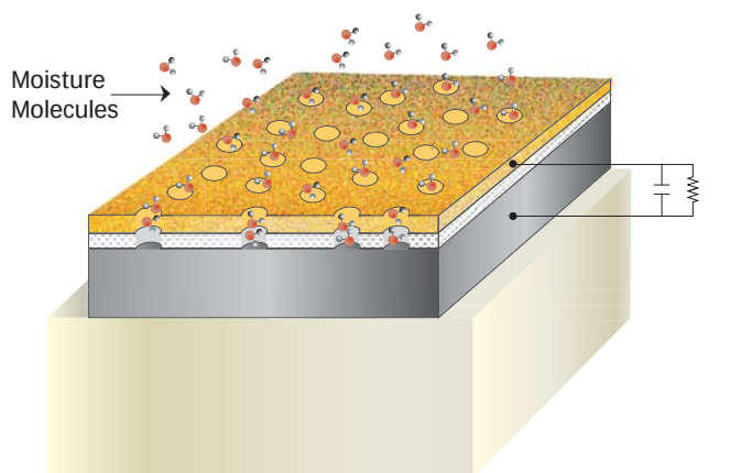
Operation of the Michell Ceramic Moisture Sensor
