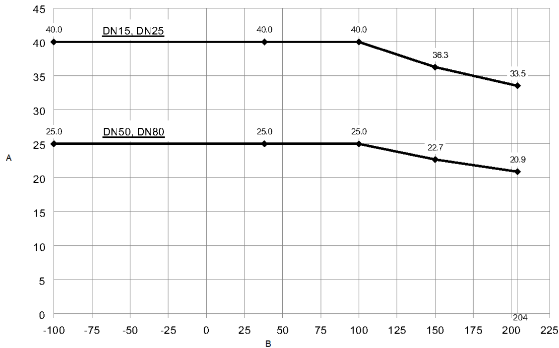
Figure 5: DIN 11851 316L hygienic coupling for H025 through H300
