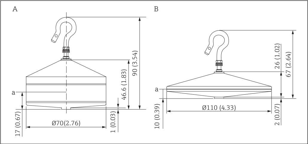
A Ø70 mm (2.76 in) 316L conical displacer B Ø110 mm (4.33 in) 316L conical displacer a Immersion point
