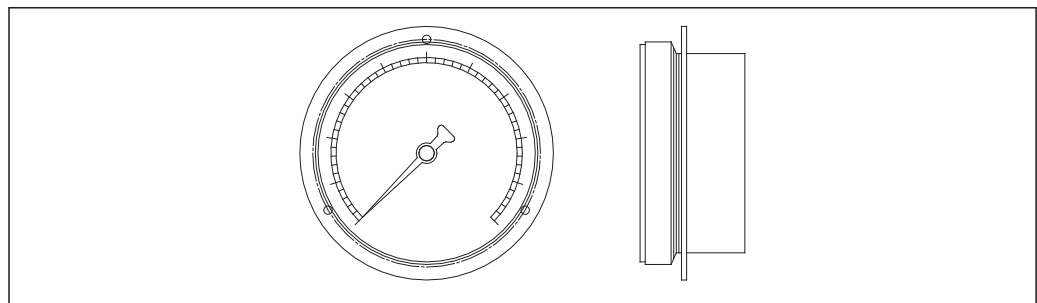
23 Pressure gauge
