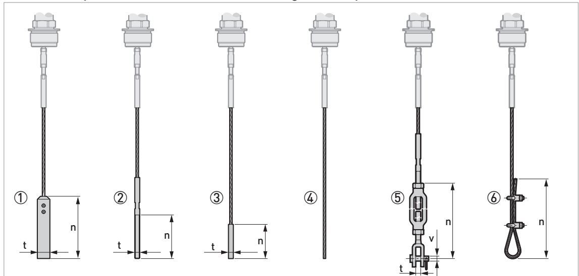
Figure 2-21: Probe end options for the Ø4 mm / 0.16" single cable probe
