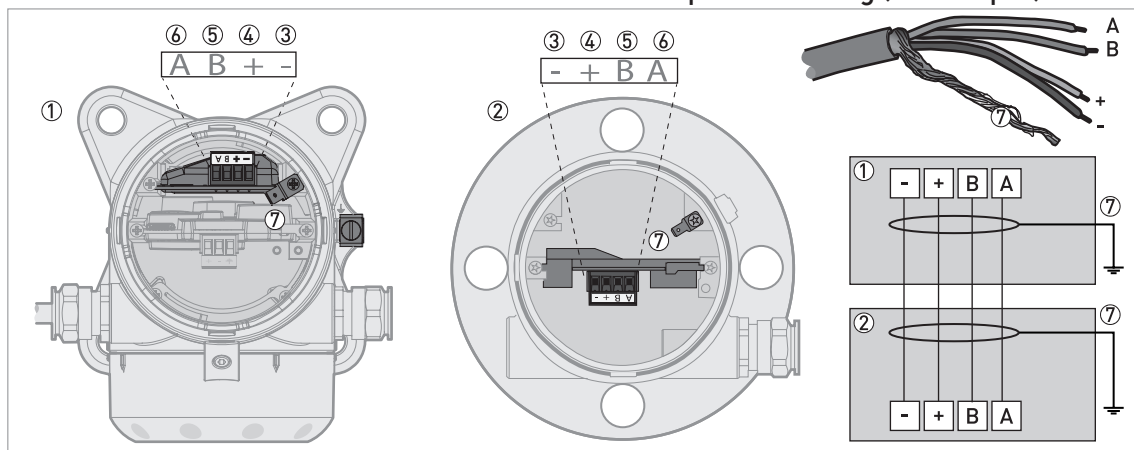
Figure 4-7: Connections between the remote converter and the probe housing (one output)
