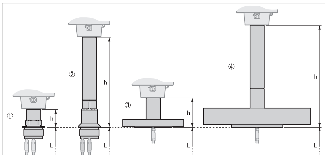
Figure 2-19: Process connection options
