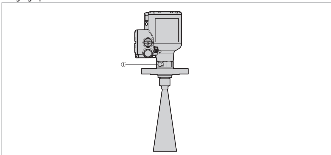
Figure 2-13: Purging options
