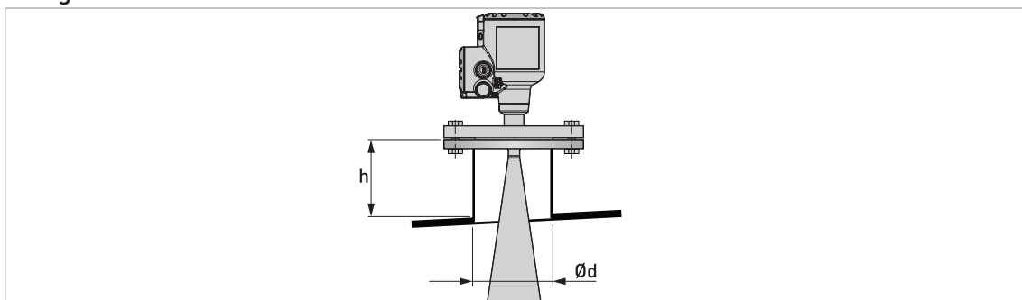
Figure 3-6: Flange connections
