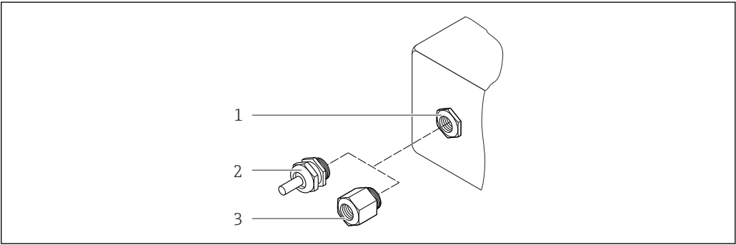
56 Possible cable entries/cable glands
