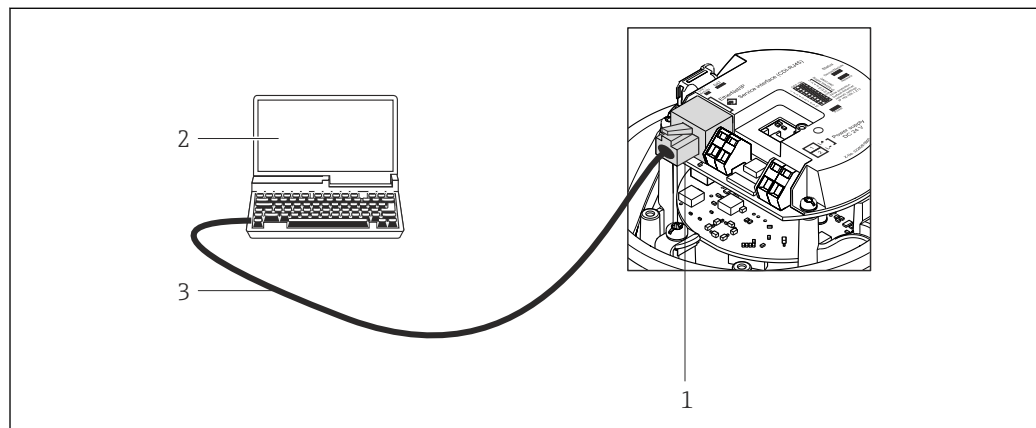
62 Connection for order code for "Output", option L: PROFIBUS DP
