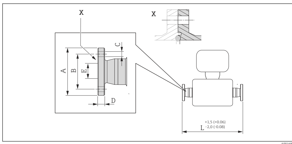
37 Detail X: Asymmetrical process connection; the part shown in gray is provided by the supplier. Engineering unit mm (in).
