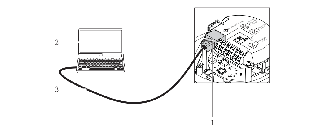
61 Connection for the order code for "Output", option B: 4-20 mA HART, pulse/frequency/switch output
