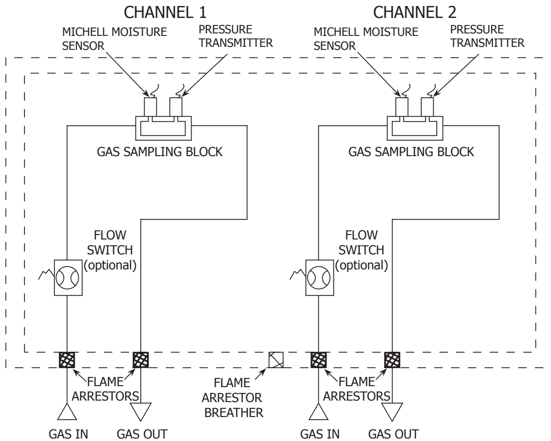
Figure 5 Pipework Connections
