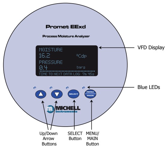
Figure 9 User Interface
