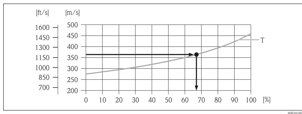
1 Calculation of the methane fraction [%] based on the sound velocity [m/s (ft/s)] and a temperature T of 40 °C (104 °F), for example.
