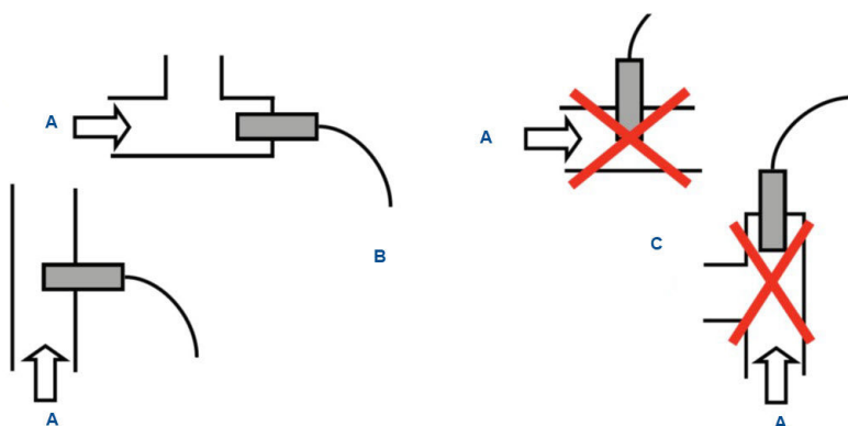
Figure 1-2: Recommended installation
