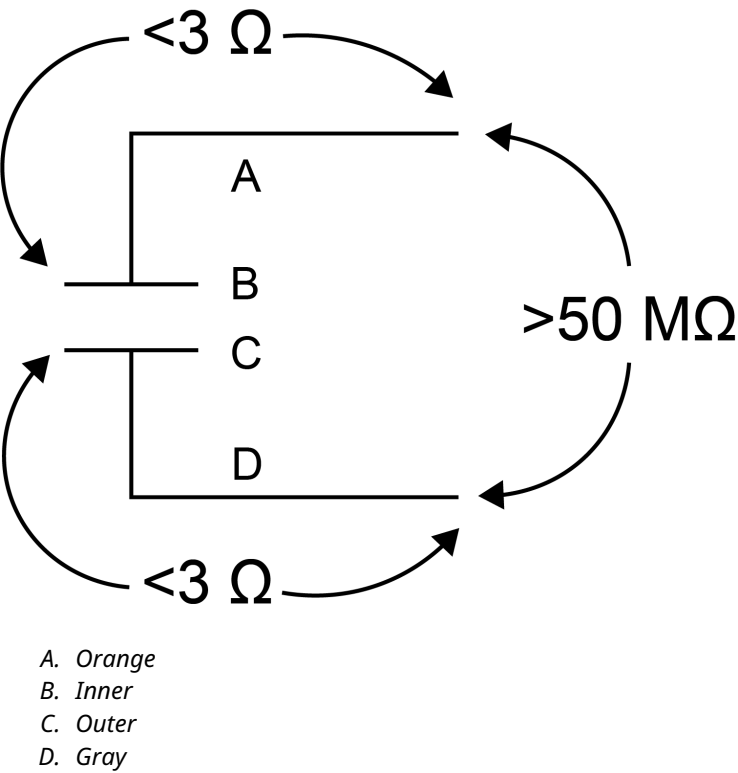
Figure 4-2: Checking the continuity and leakage
