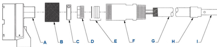
Figure 1-4: Sensor installation
