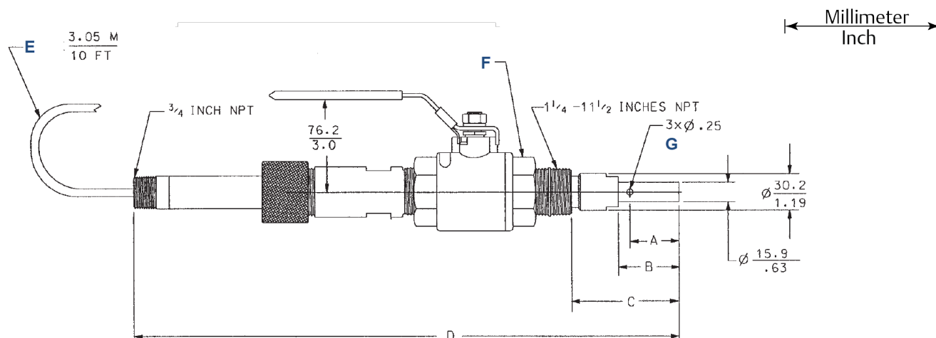
Figure 3: Rosemount 402 Dimensional Drawing
