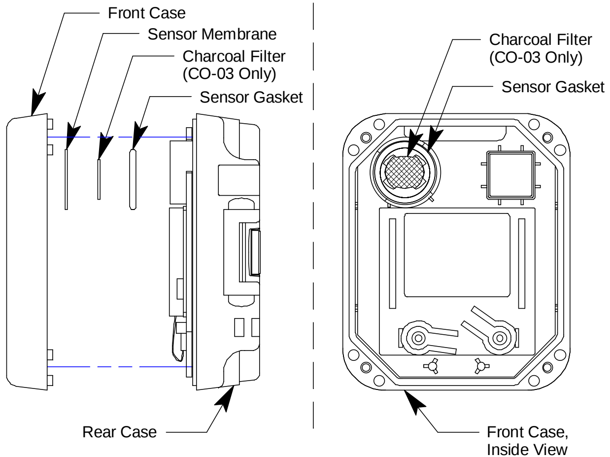
Figure 18: Replacing the Sensor Filters
