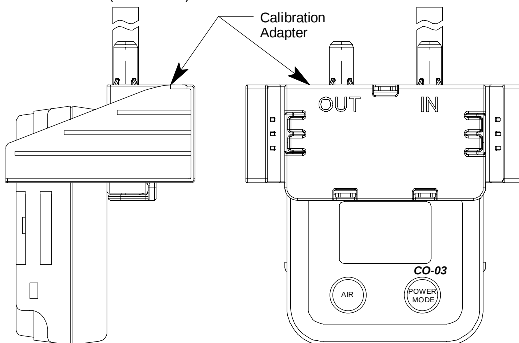
Figure 10: Installing the Calibration Adapter
