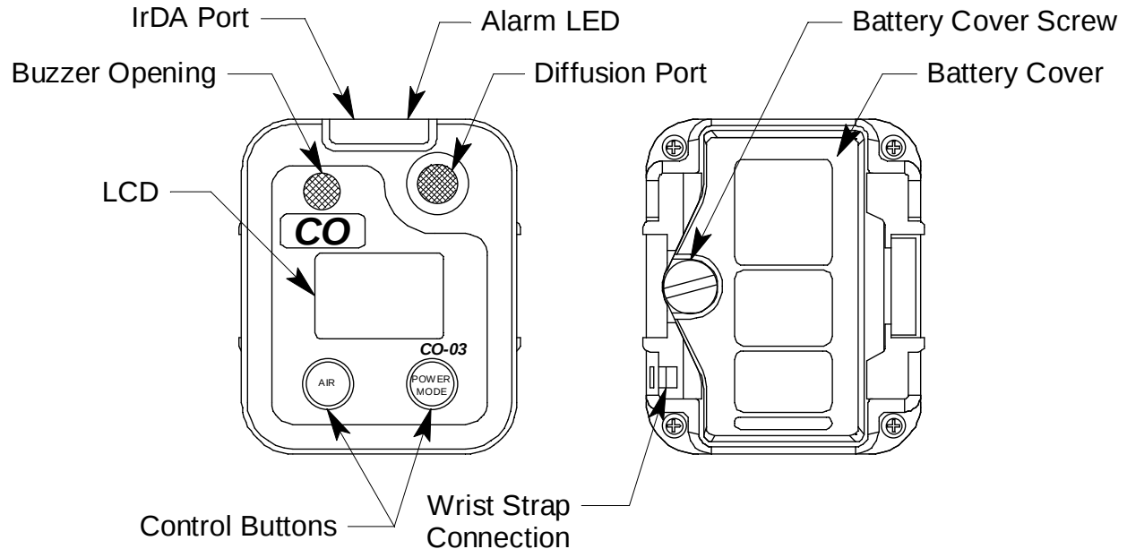
Figure 1: Components of the 03 Series
