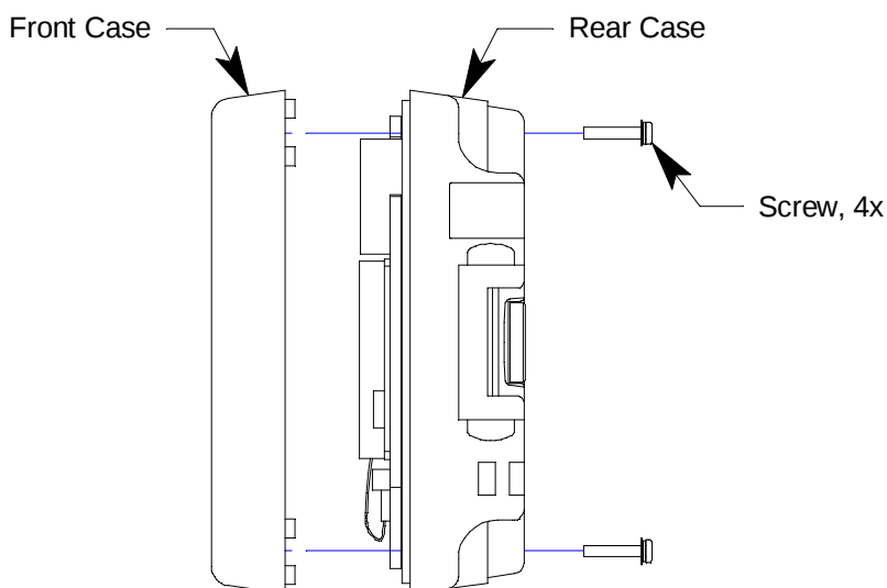
Figure 17: Case Separation
