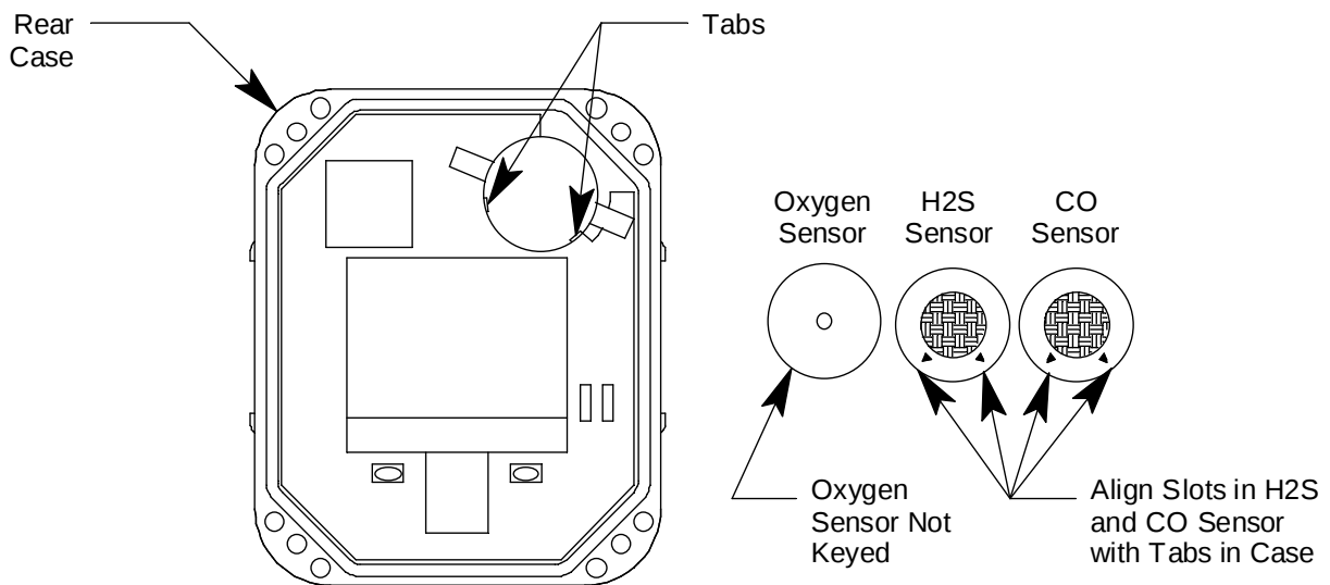
Figure 16: Replacing the Sensor
