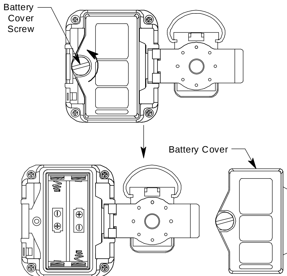
Figure 14: Removing the Battery Cover
