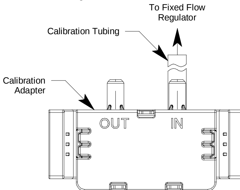
Figure 11: Calibration Kit Assembly
