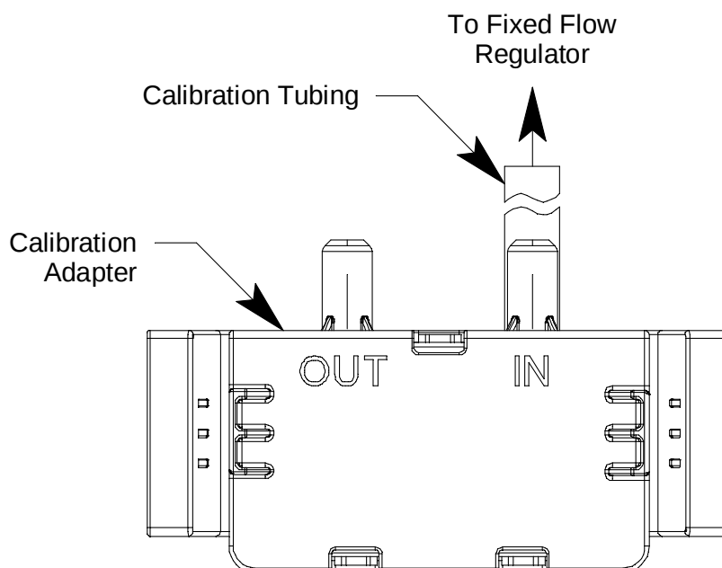
Figure 9: Calibration Kit Assembly
