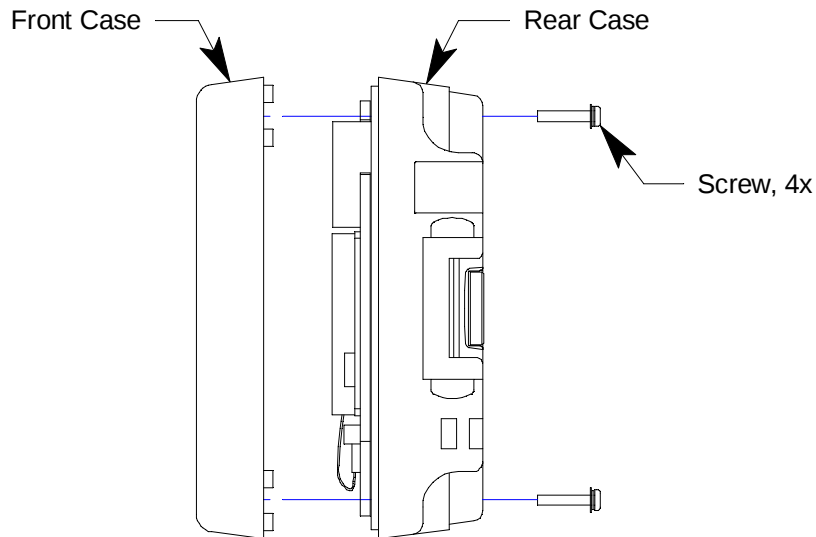
Figure 15: Case Separation
