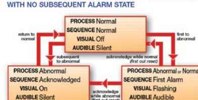
AUTOMATIC RESET FIRST OUT WITH NO SUBSEQUENT ALARM STATE Sequence F1A
