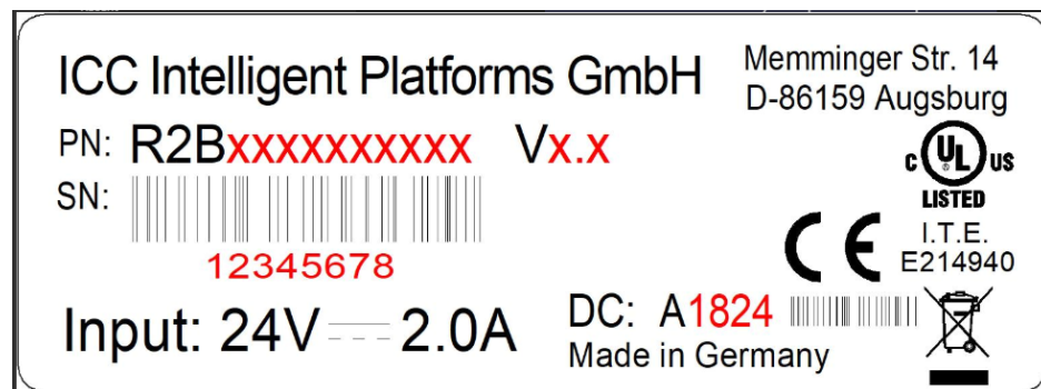
Figure 29: UL Label
