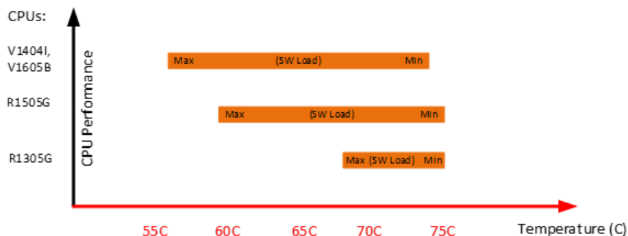
Figure 28: Upper Ambient Air Temperature Limit Range
