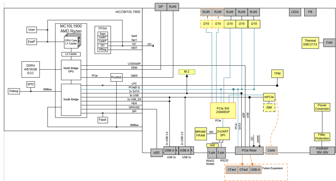
Figure 16: Overview of the Interface Usage
