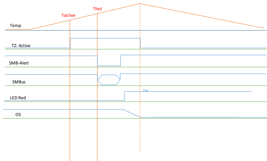
Figure 26: Thermal Zones: Tactive to Thot
