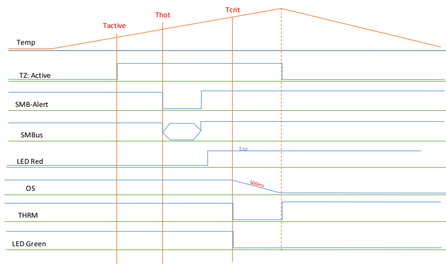
Figure 27: Thermal Zone Tactive to Thot to Tcrit
