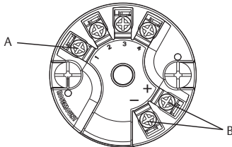
A. Sensor terminals B. Power/communication terminals
