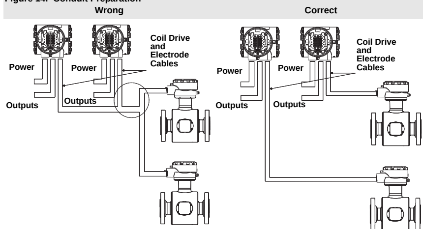
Figure 14. Conduit Preparation
