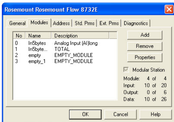
Figure 23. Basic Slot Configuration
