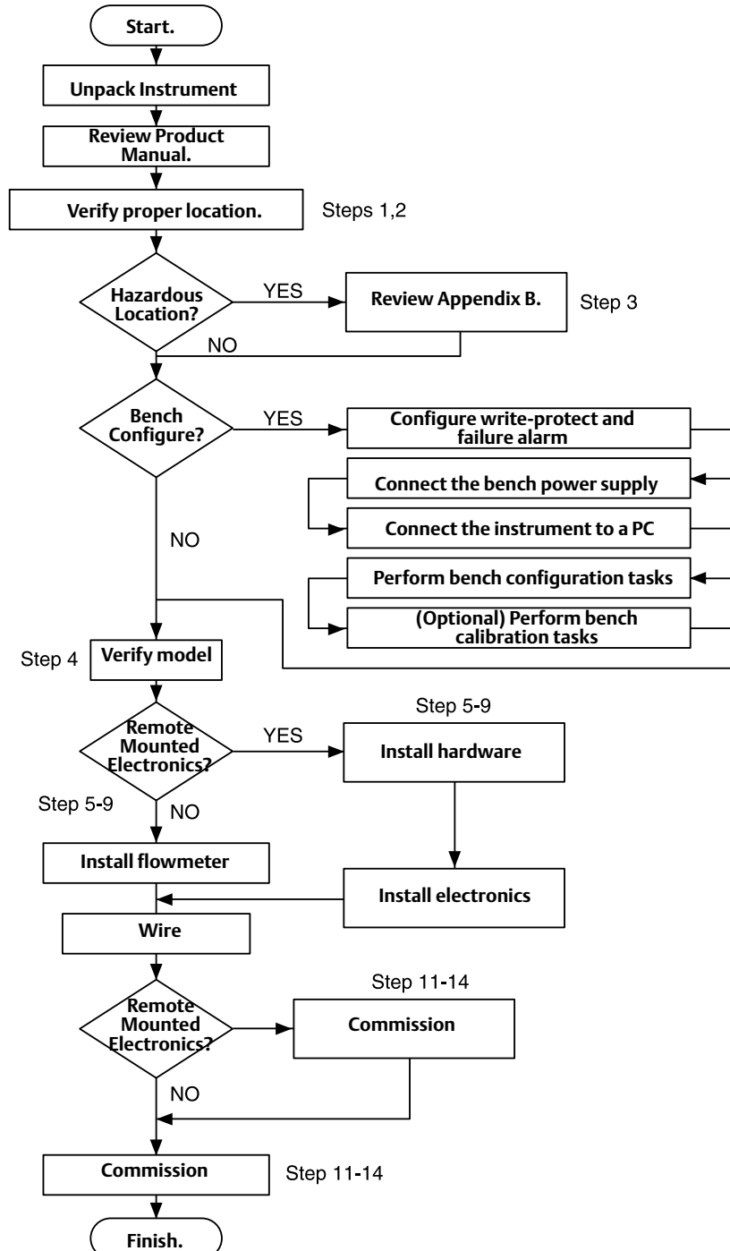
Figure 2-1. Commissioning Chart
