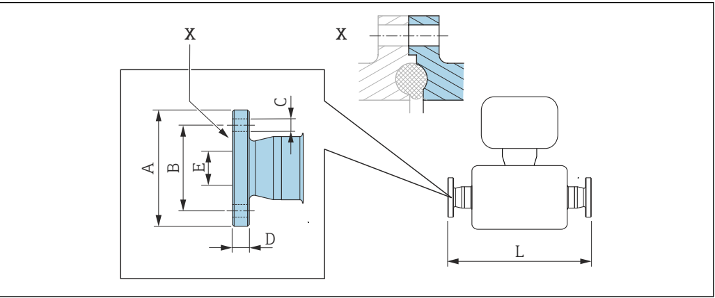
40 Detail X: Asymmetrical process connection; the part shown in gray is provided by the supplier.
