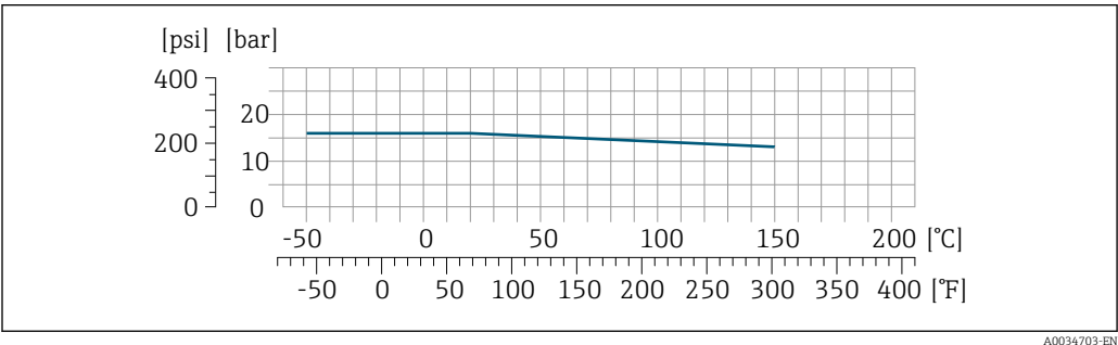
36 With connection material 1.4435 (316L)
