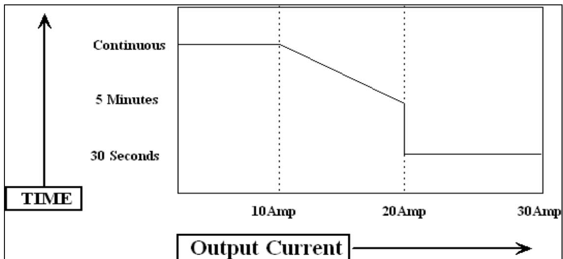
Graph 1* : Operating time on 30A range with current into a short circuit at 20°C Continuous current is available up to 10A output.
