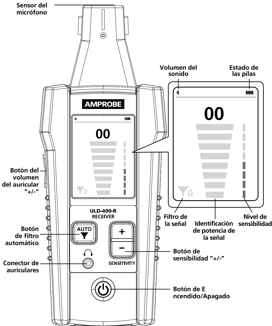
Figura 3.2: Receptor ULD-400-R
