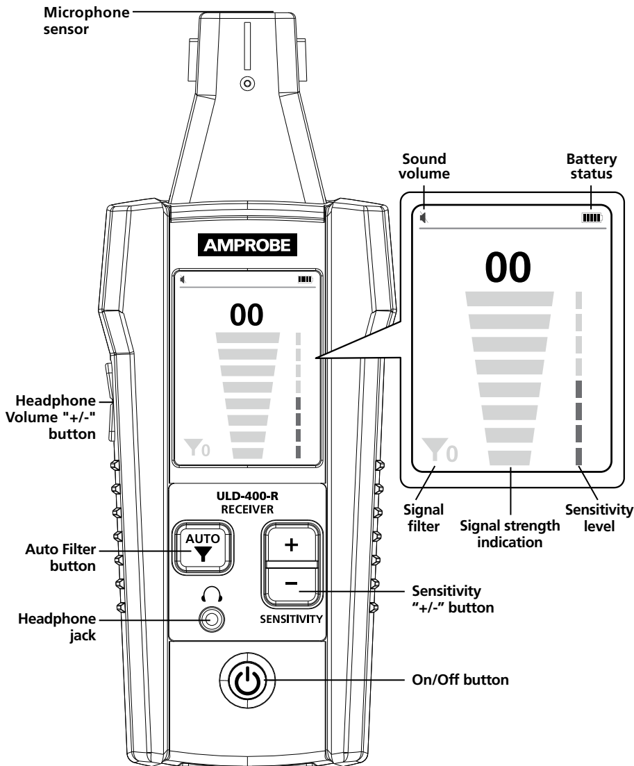
Figure 3.2: ULD-400-R Receiver
