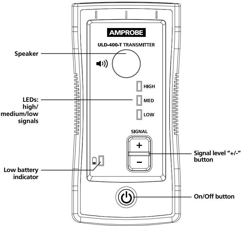
Figure 3.3: ULD-400-T Transmitter
