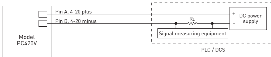
Typical circuit
