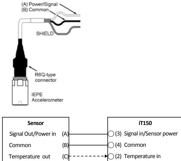
Figure 6 - Sensor connections
