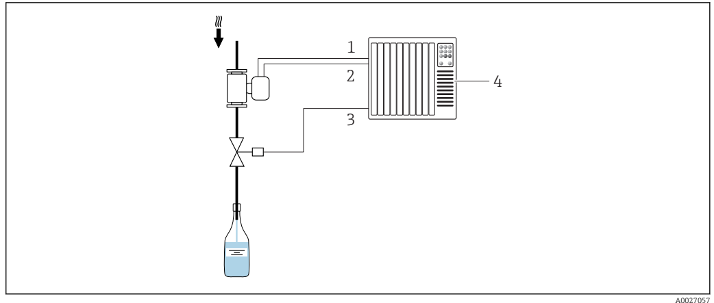
1 Options for integration into a system for batching processes
