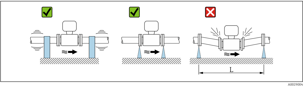
11 Measures to avoid device vibrations ( L > 10\text{ m} (33 ft))
