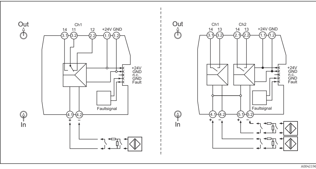
8 Terminal assignment of RLN22: 1-channel version (left), 2-channel version (right)
