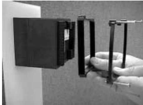
Figure 8.3b — Retention Collar and Mounting Bracket.
