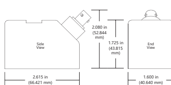
SE16A, SE16B, & SE16C Transducers & Mounting
