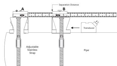
SE16A, SE16B, & SE16C Transducers & Mounting
