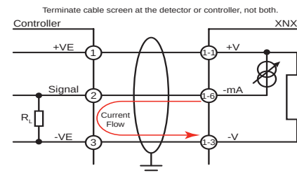
Figure 35. Source wiring
