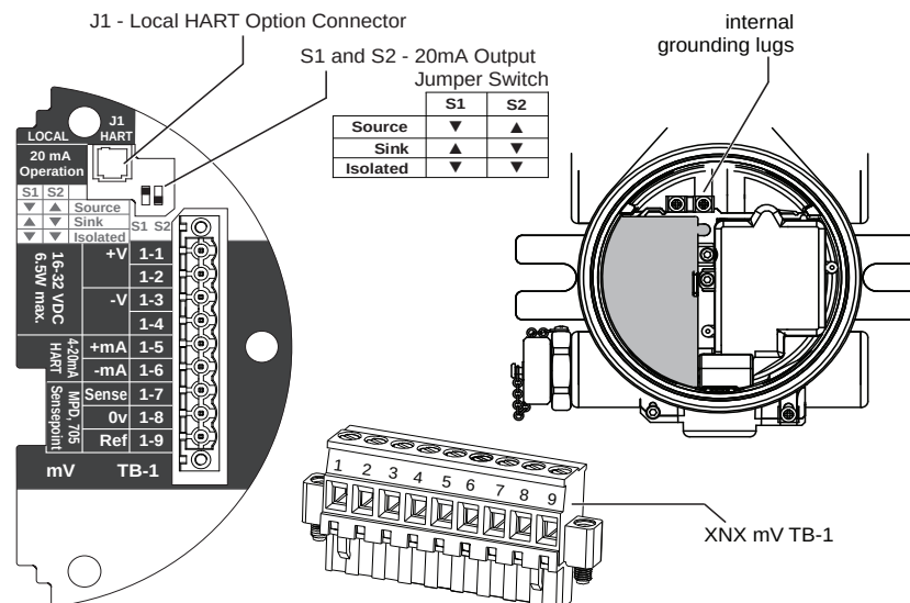
Figure 43. mV personality board terminal blocks and jumper switches
