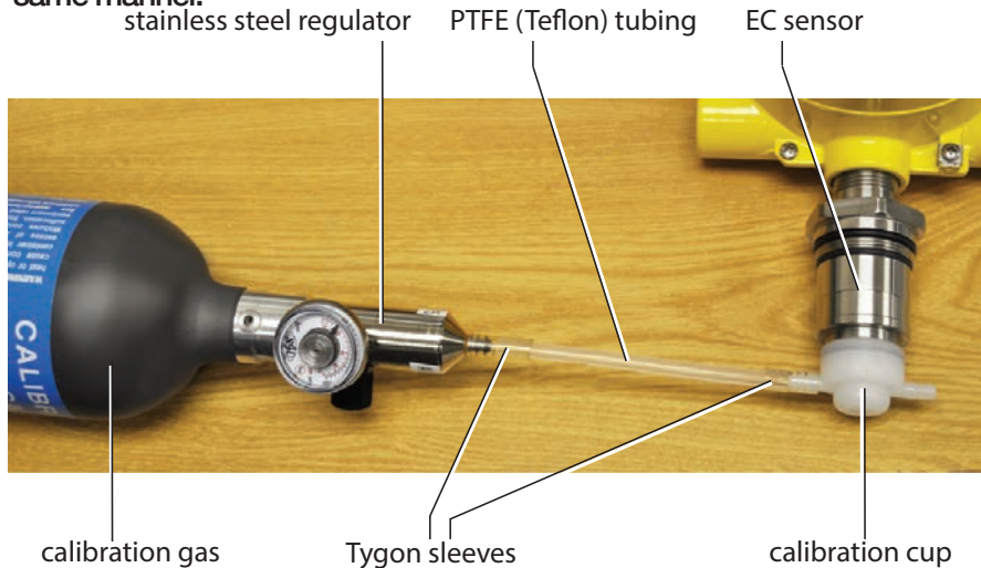
Figure 192. Joining the PTFE tubing with Tygon tubing
