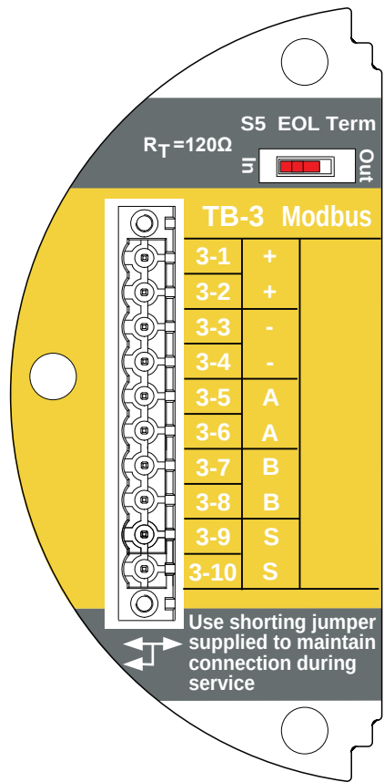
Figure 246. Modbus connections
