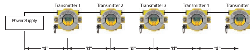
Figure 31. Daisy-chained transmitter distances
