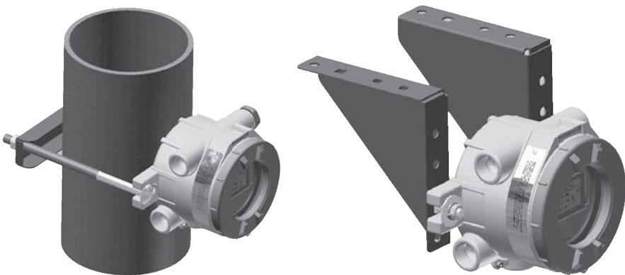
Figure 25. Optional pipe and ceiling mounts
