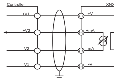
Figure 36. Isolated wiring
