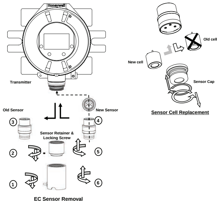
Figure 227. XNX EC sensor and cell replacement
