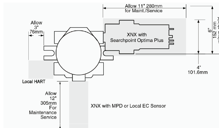
Figure 22. XNX Universal Transmitter mounting dimensions and clearances
