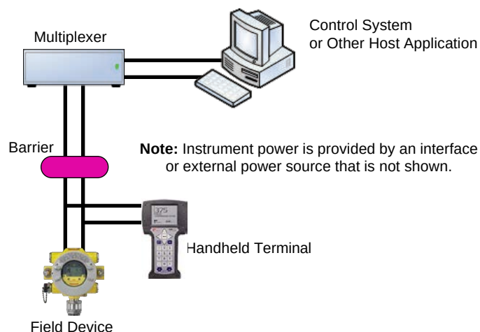
Figure 55. Point-to-point mode of operation
