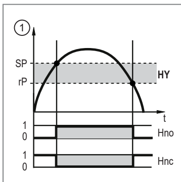
Fig. 8: Hysteresis function
