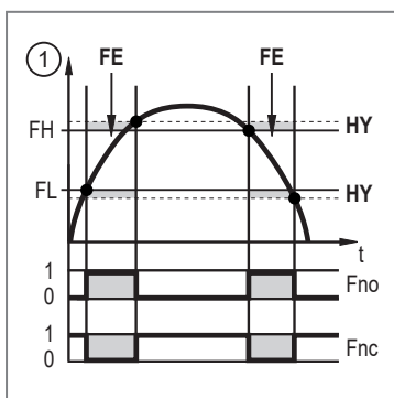
Fig. 9: Window function
