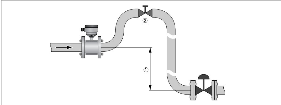
Figure 3-11: Air venting
