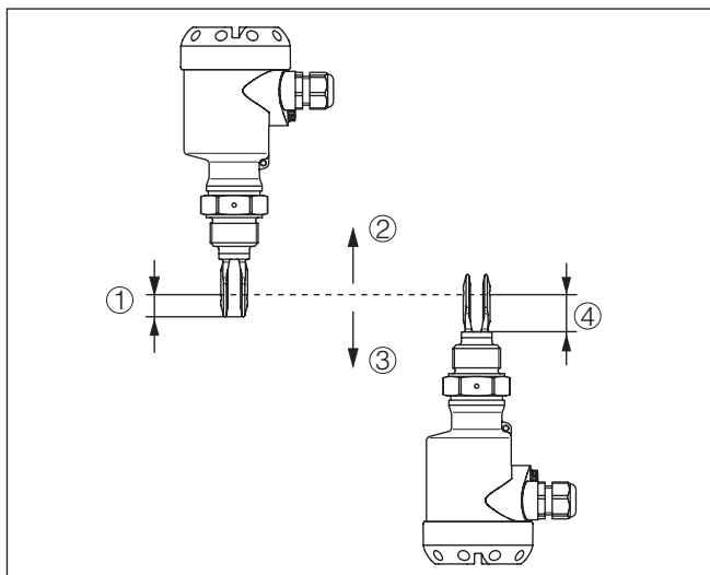
Fig. 2: Vertical mounting
