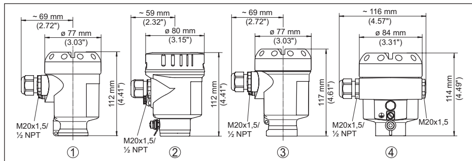
Fig. 32: Housing versions
