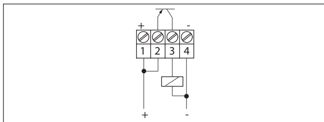
Fig. 14: PNP action
