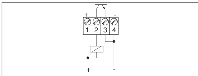
Fig. 13: NPN action
