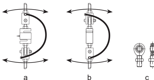
Figure 11-2. ITCM Weigh Module
