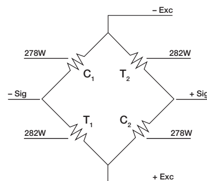
Figure 25-2. Wheatstone Bridge
