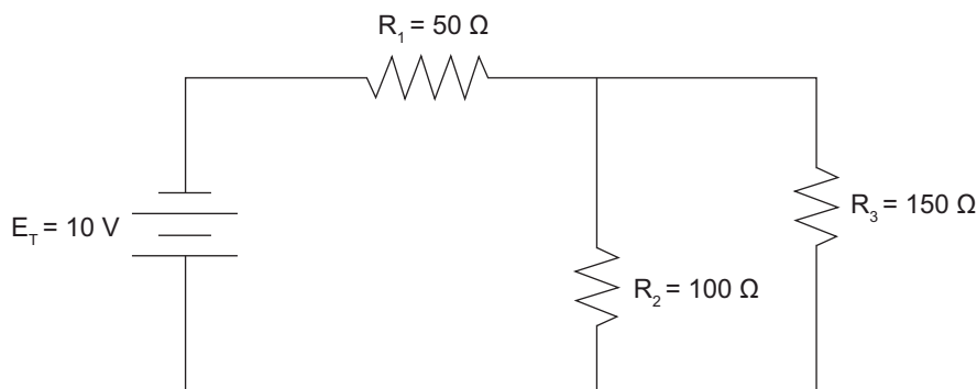
Figure 5-6. Series-Parallel Circuit
