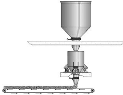
Figure 12-6. Storage Silo Fed Weigh Hopper
