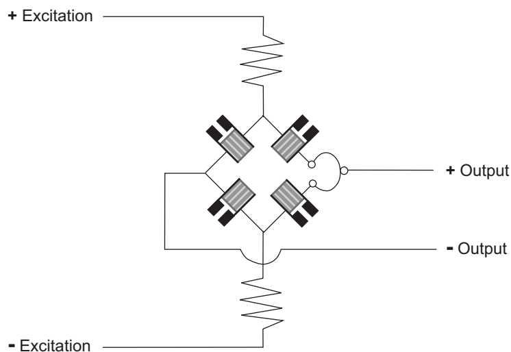
Figure 5-13. Load Cell
