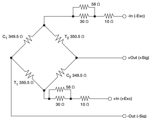
Figure 6-2. Wheatstone Bridge
