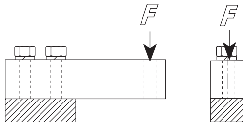
Figure 8-1. Single-Ended Beam
