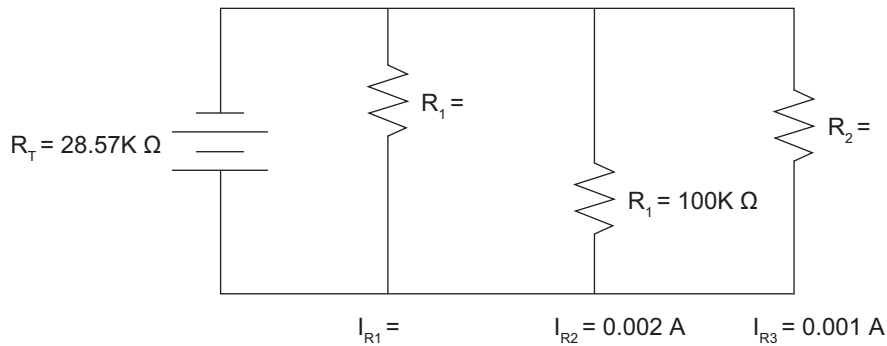
Figure 5-5. Parallel Resistive Circuit
