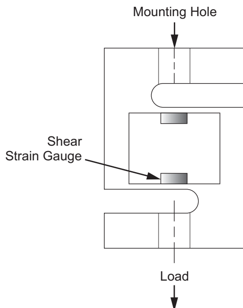
Figure 1-5. S-Beam
