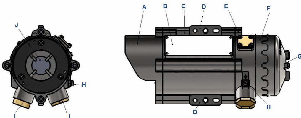
Figure 2-1: Flash source
