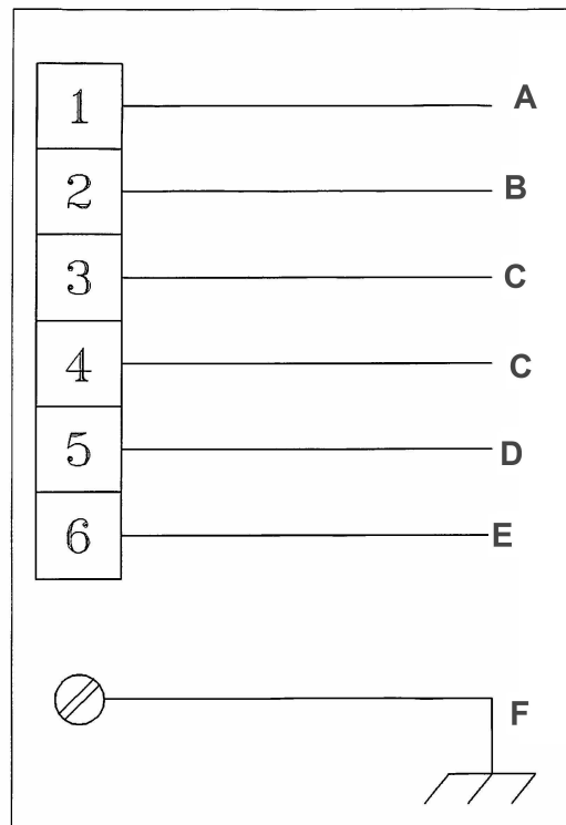
Figure A-2: Source Wiring Terminal
