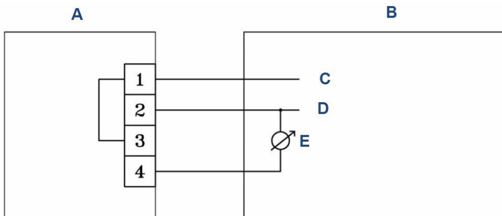
Figure A-5: 0-20 mA Source 3 Wire
