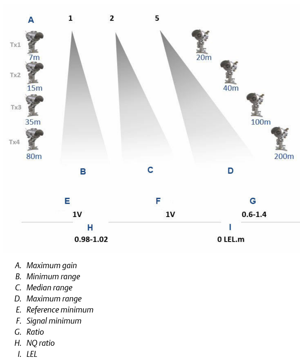
Figure 6-2: Maintenance Channels' Limits
