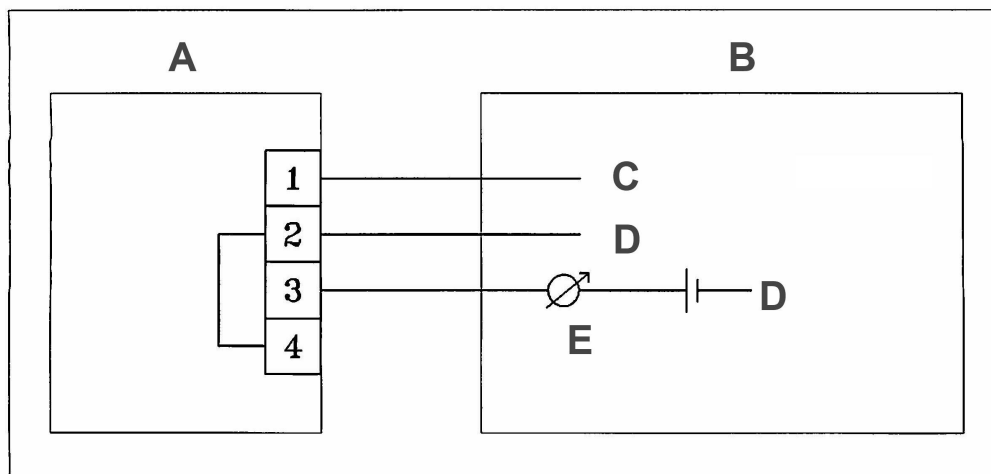
Figure A-4: 0-20 mA Non-Isolated Sink 3 Wire
