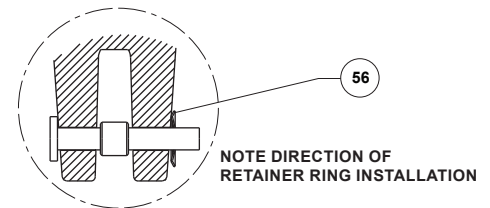
RETAINER RING INSTALLATION DETAILS
