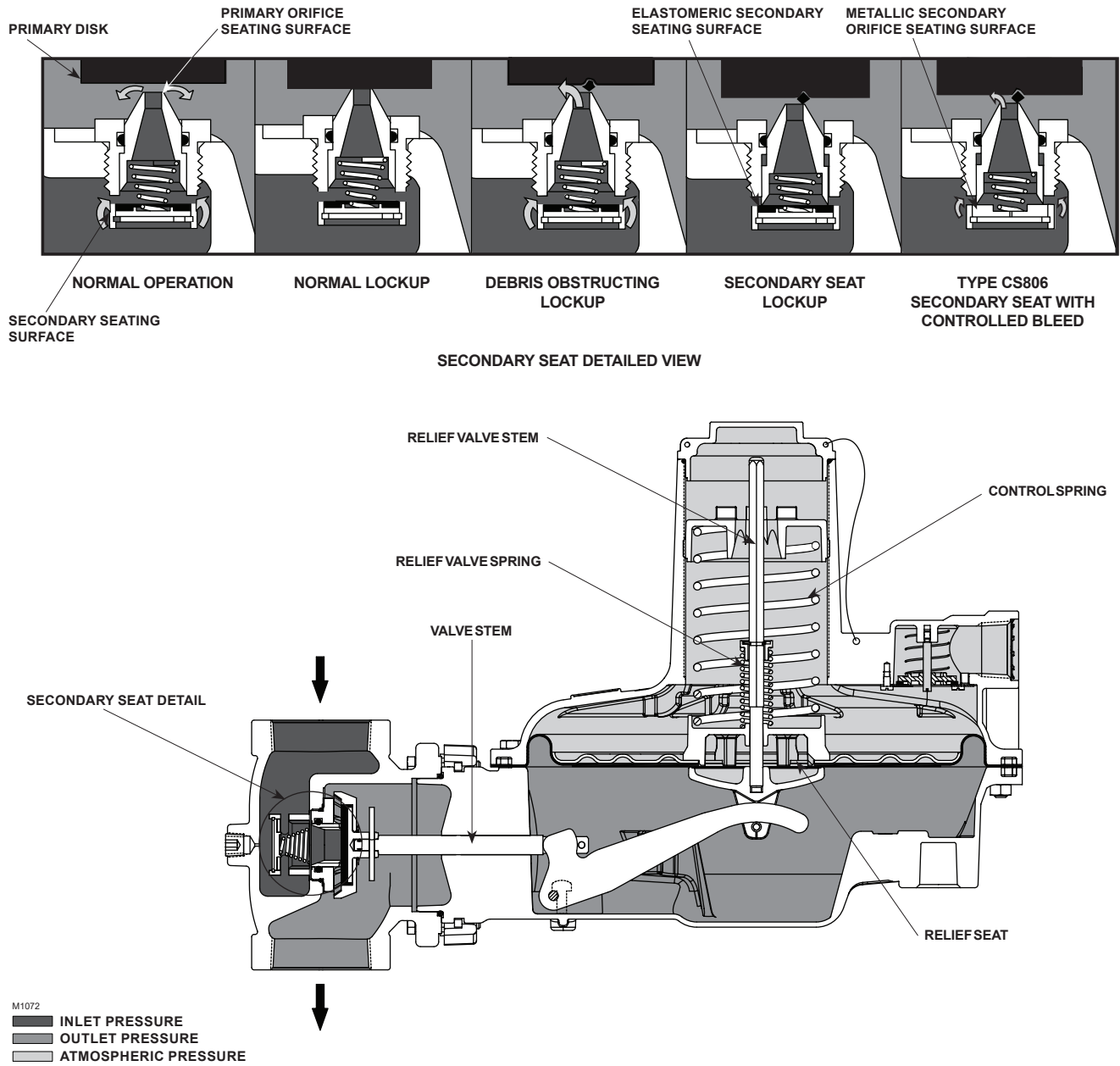
Figure 6. Type CS805IR with Secondary Seat Protection
