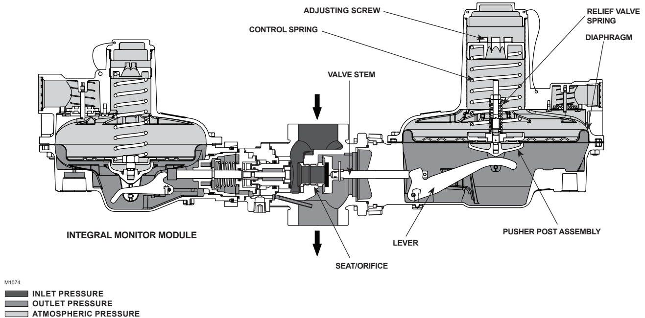
Figure 4. Type CS803IT Internally Registered Primary Regulator with Internally Registered Integral Monitor Operational Schematic
