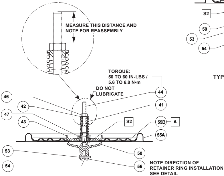
TYPE CS800/CS820 STANDARD FLOW TOKEN RELIEF
