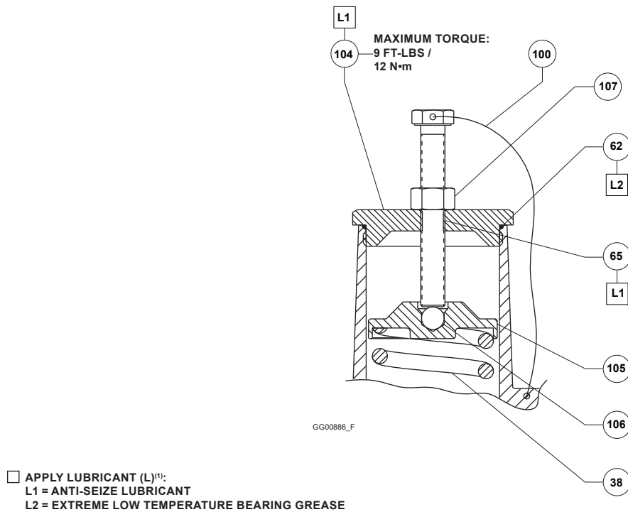
Figure 17. CS800 Series Control Spring Adjustment Assemblies (continued)
