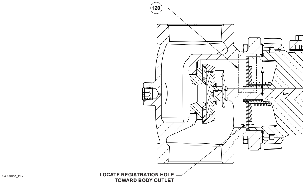
Figure 14. CS800 Series with Stabilizer Cartridge Assembly
