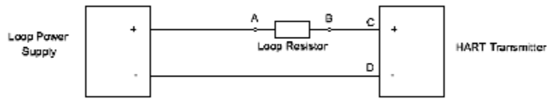
Figure 1. HART Connections
