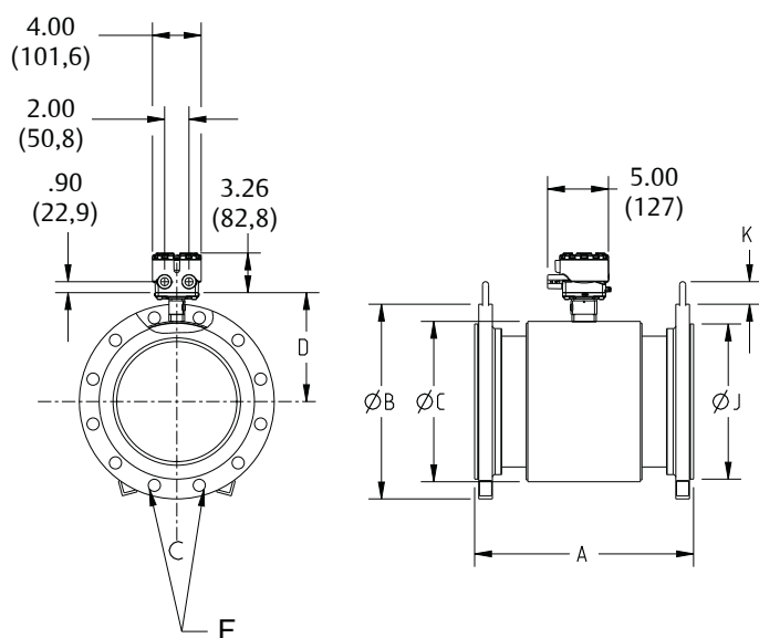
Figure 12: Raised face flanged sensor 3-in to 48-in. (75 mm to 1200 mm)
