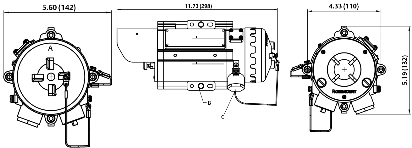
Figure 2: Source Assembly
