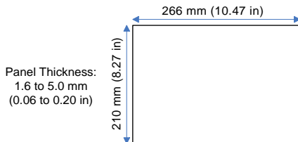
Figure 4.9: IC755CxS10CDx Panel Cutout Dimensions
