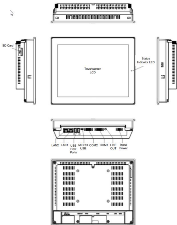
Figure 1.3: IC755CxS10CDx Profile and Hardware Features
