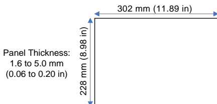
Figure 4.10: IC755CxS12CDx Panel Cutout Dimensions
