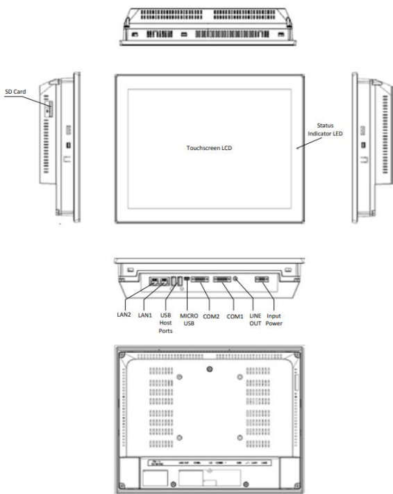
Figure 1.4: IC755CxS12CDx Profile and Hardware Features
