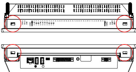
Figure 4.4: IC755CxS10CDx Mounting Holes
