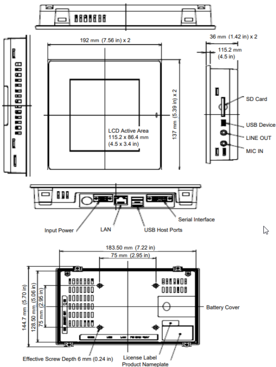
Figure 1.1: IC755CxS06RDx Profile and Hardware Features
