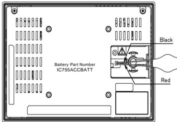
Figure 3.2: IC755CxS06RDx /IC755CxW07CDx Battery Harness Connection
