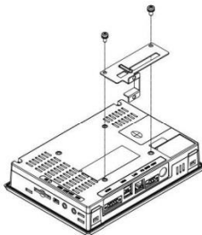
Figure 5.4: USB retaining Clamp Plate
