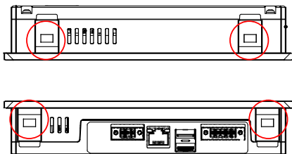
Figure 4.2: IC755CxS06RDx Mounting Holes
