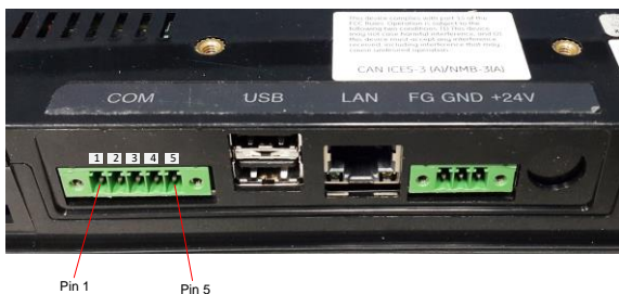
Figure 4.3: IC755CxW07CDx Serial Port COM1 Pin-out
