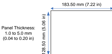
Figure 4.8: IC755CxW07CDx Panel Cutout Dimensions
