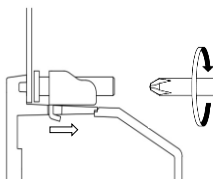
Figure 4.14: Mounting bracket screw turning
