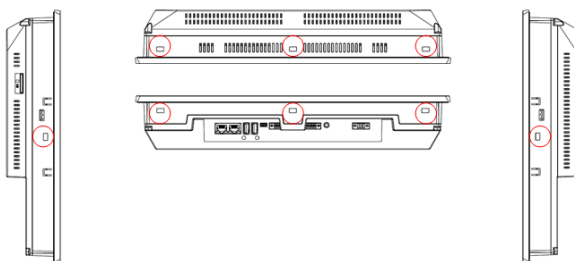
Figure 4.6: IC755CxS15CDx Mounting Holes
