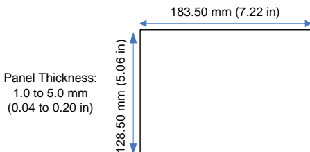
Figure 4.7: IC755CxS06RDx Panel Cutout Dimensions
