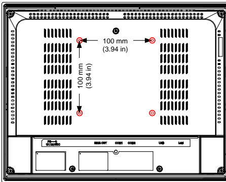
Figure 4.16: IC755CxSxxCDx VESA Mounting Holes
