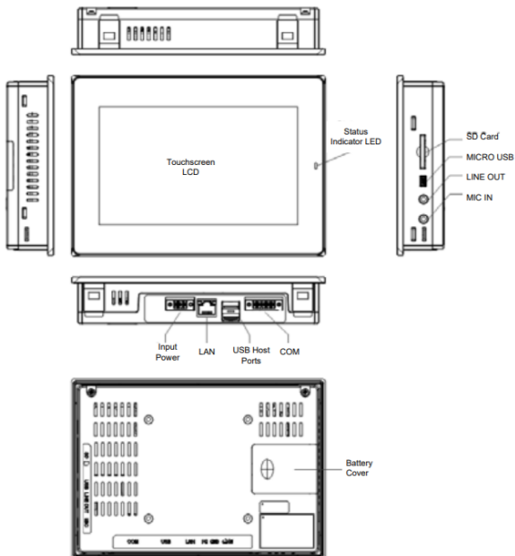
Figure 1.2: IC755CxW07CDx Profile and Hardware Features
