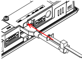
Figure 5.5: USB cable retaining clamp
