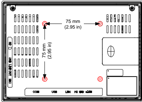
Figure 4.16: IC755CxSxxCDx VESA Mounting Holes
