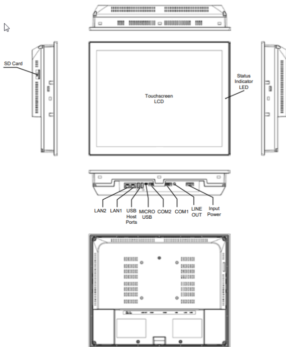
Figure 1.5: IC755CxS15CDx Profile and Hardware Features
