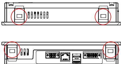
Figure 4.3: IC755CxW07CDx Mounting Holes
