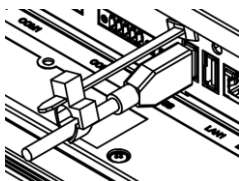
Figure 5.2: USB Retaining Clamp
