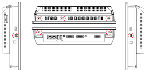
Figure 4.5: IC755CxS12CDx Mounting Holes
