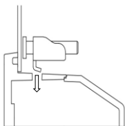
Figure 4.13: Hook of Mounting Bracket
