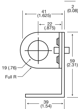
Adjustable Mounting Bracket
