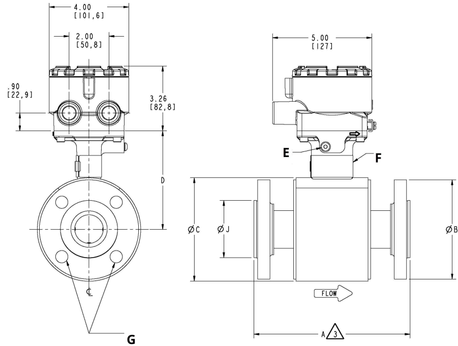
Figure 19: 8705-M Flanged Sensor ½ in. to 24 in. (DN 15 mm to 600 mm) slip-on flange - high pressure ( P \leq \text{Class 900} )
