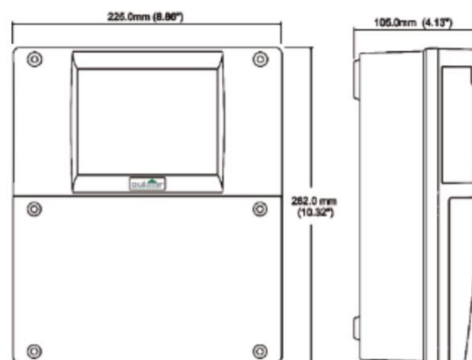
Ultimate Controller wall mount drawing front and side
