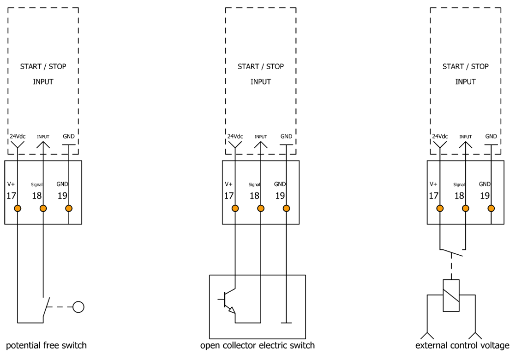
Figure: Three possible variants for connecting a reset switch
